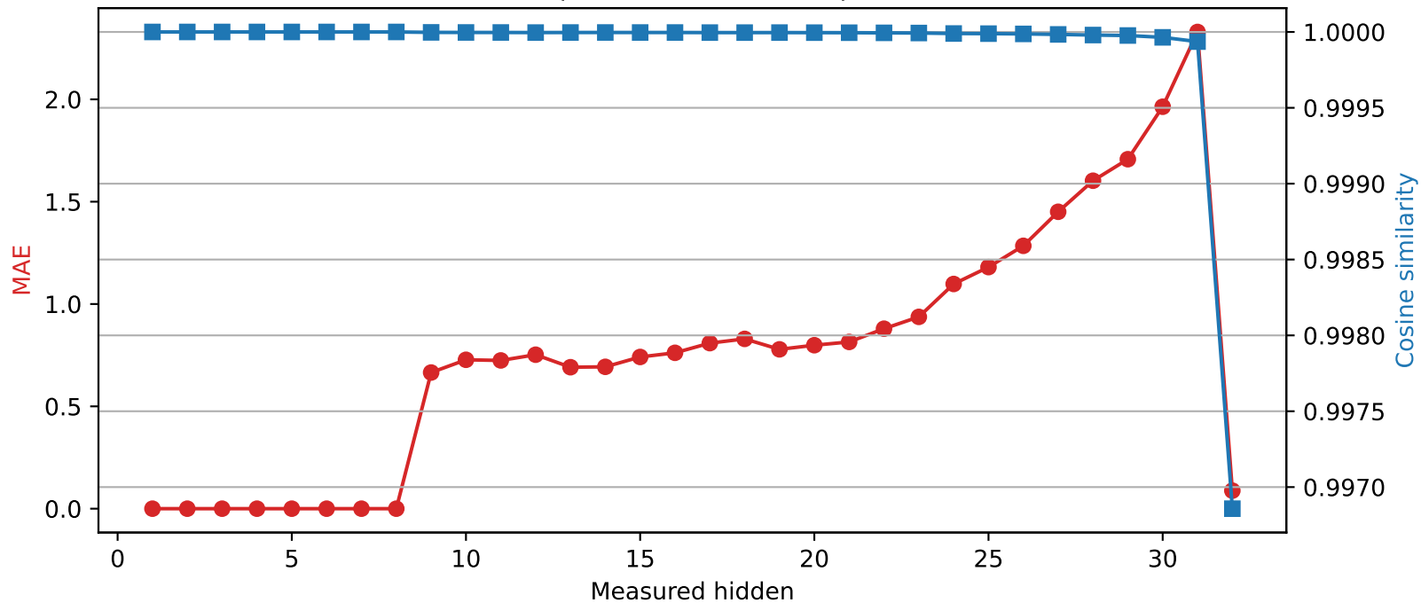
SmolLM2-360M | Quantized layer 8 | float32 → int2
