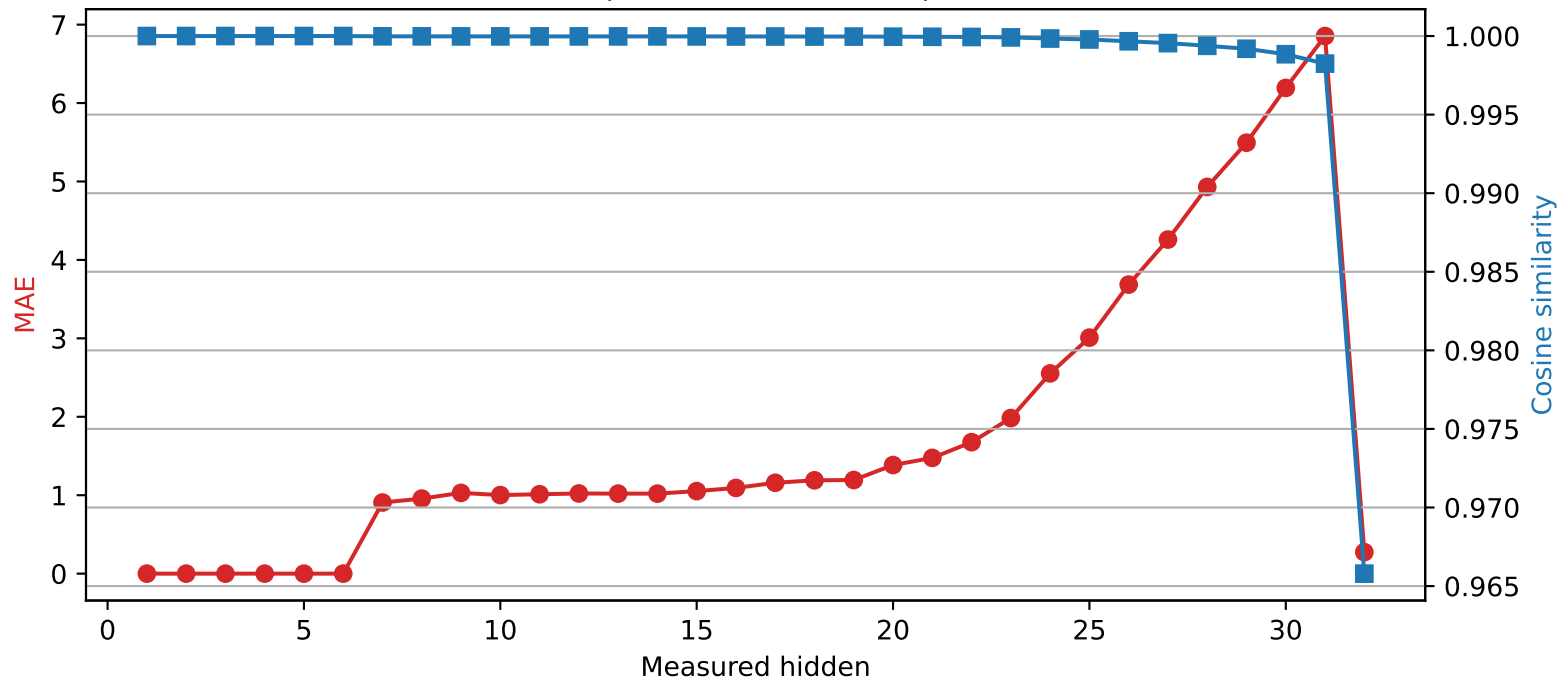
SmolLM2-360M | Quantized layer 6 | float32 \rightarrow int2
