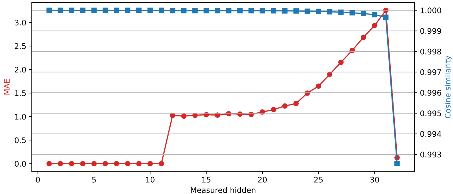
SmolLM2-360M | Quantized layer 11 | float32 → int2
