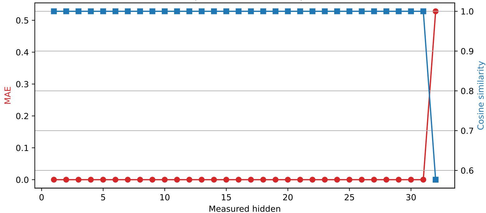
SmolLM2-360M | Quantized layer 31 | float32 → int2
