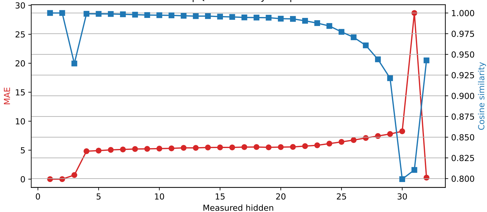
SmolLM2-360M | Quantized layer 2 | float32 → int2
