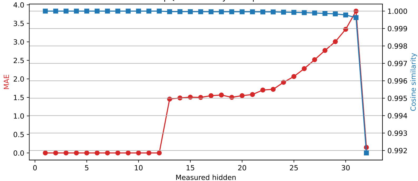
SmolLM2-360M | Quantized layer 12 | float32 → int2
