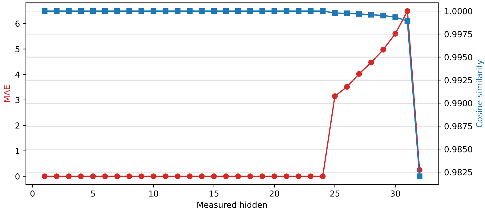
SmolLM2-360M | Quantized layer 24 | float32 → int2
