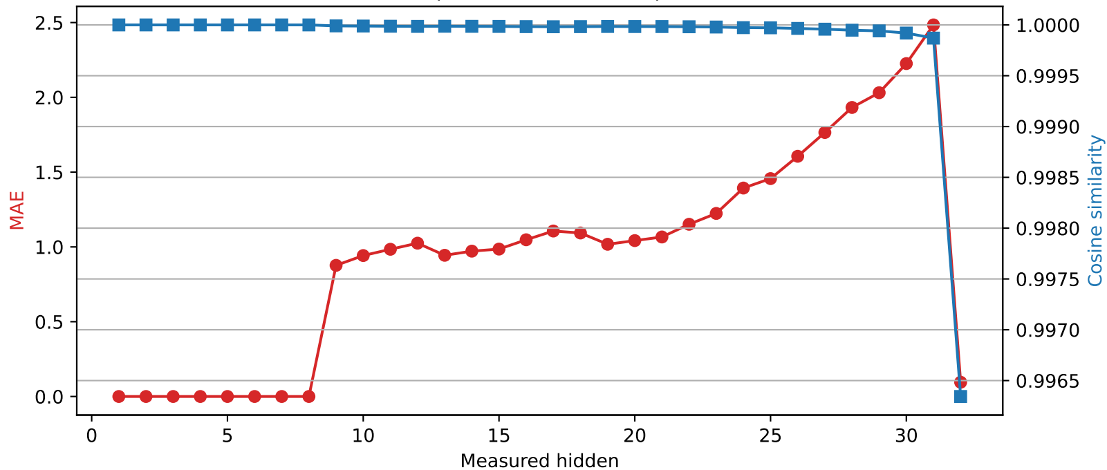
SmolLM2-360M | Quantized layer 8 | float32 \rightarrow int2
