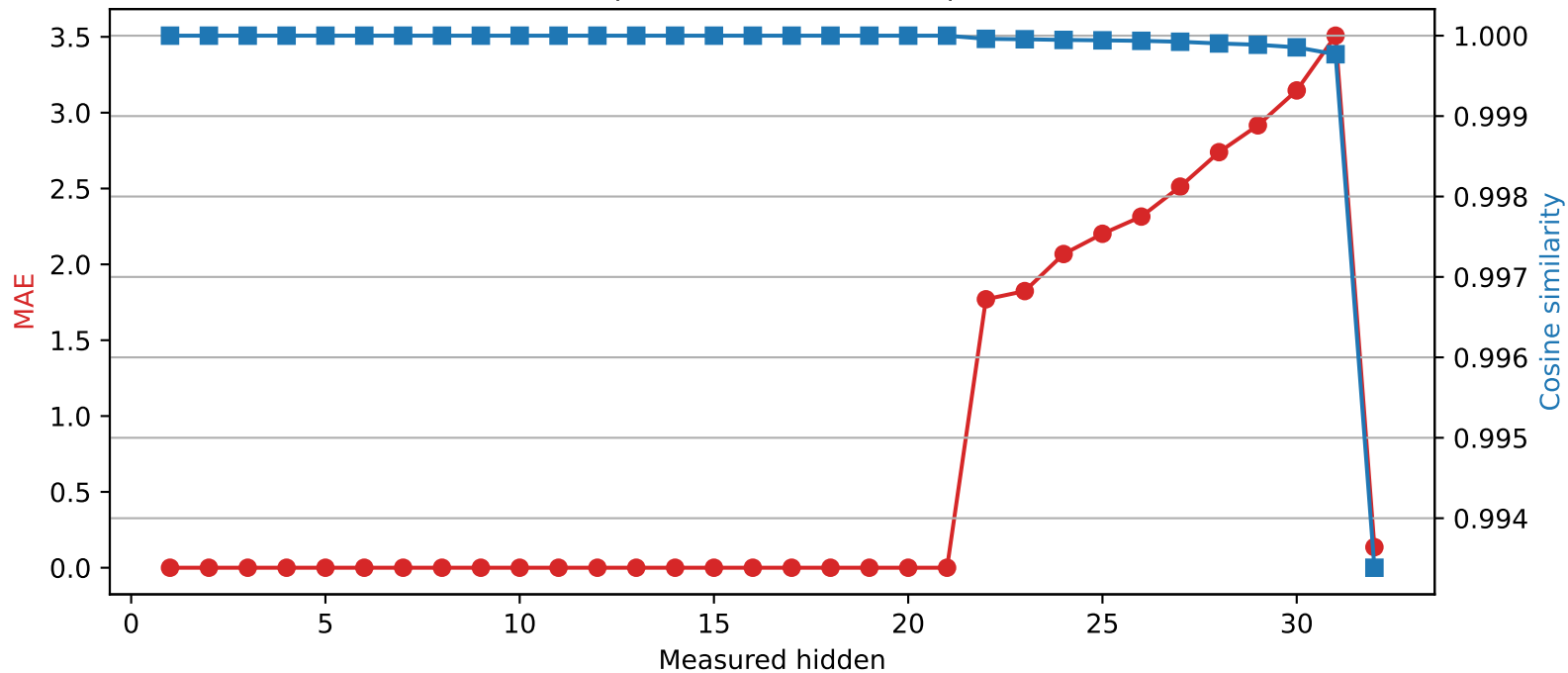
SmolLM2-360M | Quantized layer 21 | float32 \rightarrow int2
