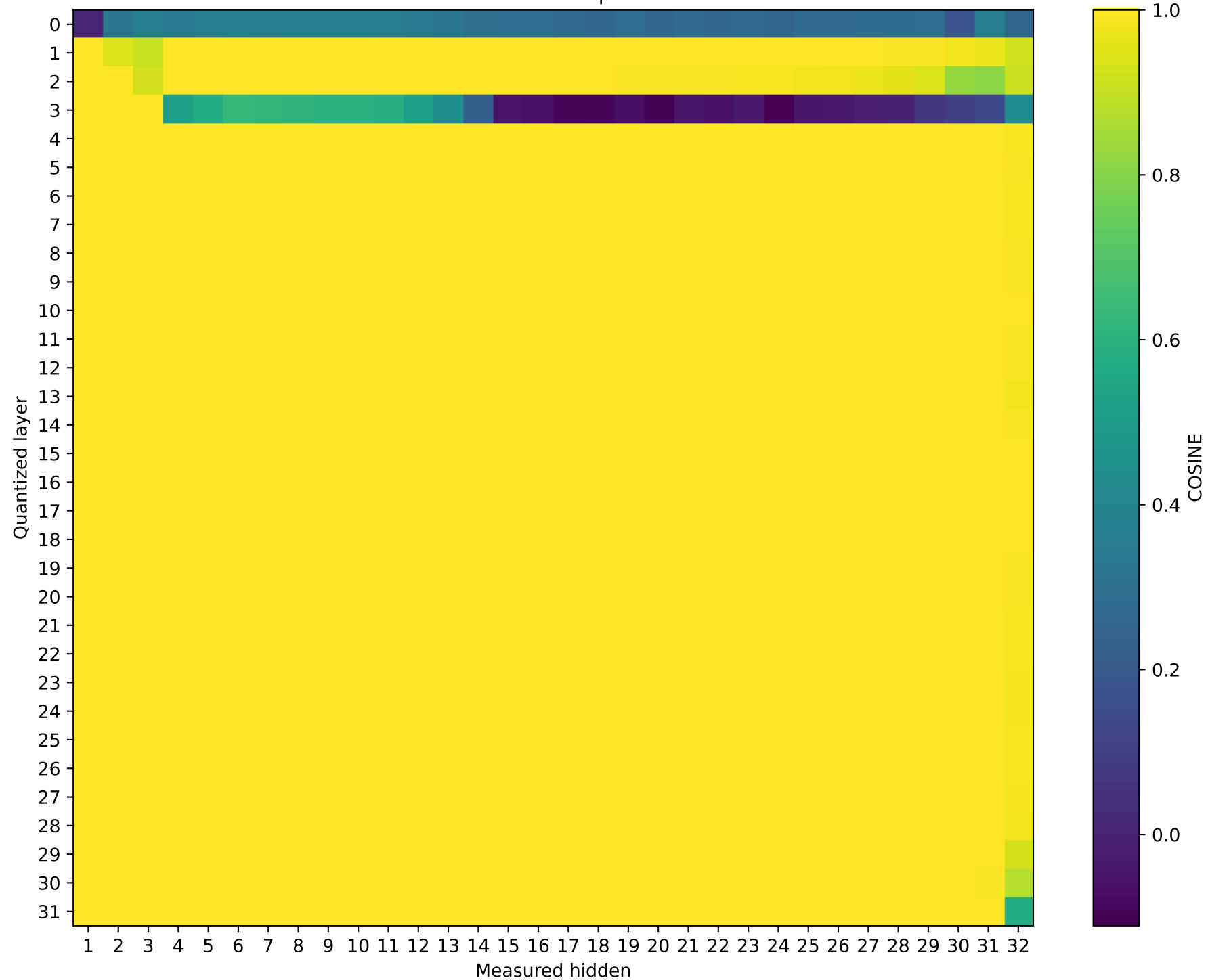
Model: SmolLM2-360M | float64 → int2
