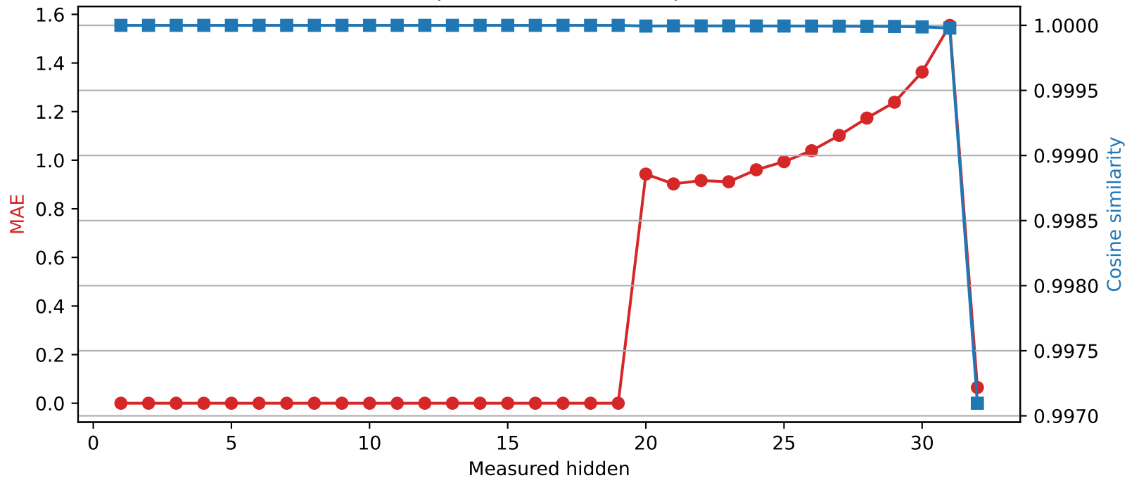
SmolLM2-360M | Quantized layer 19 | float64 → int2
