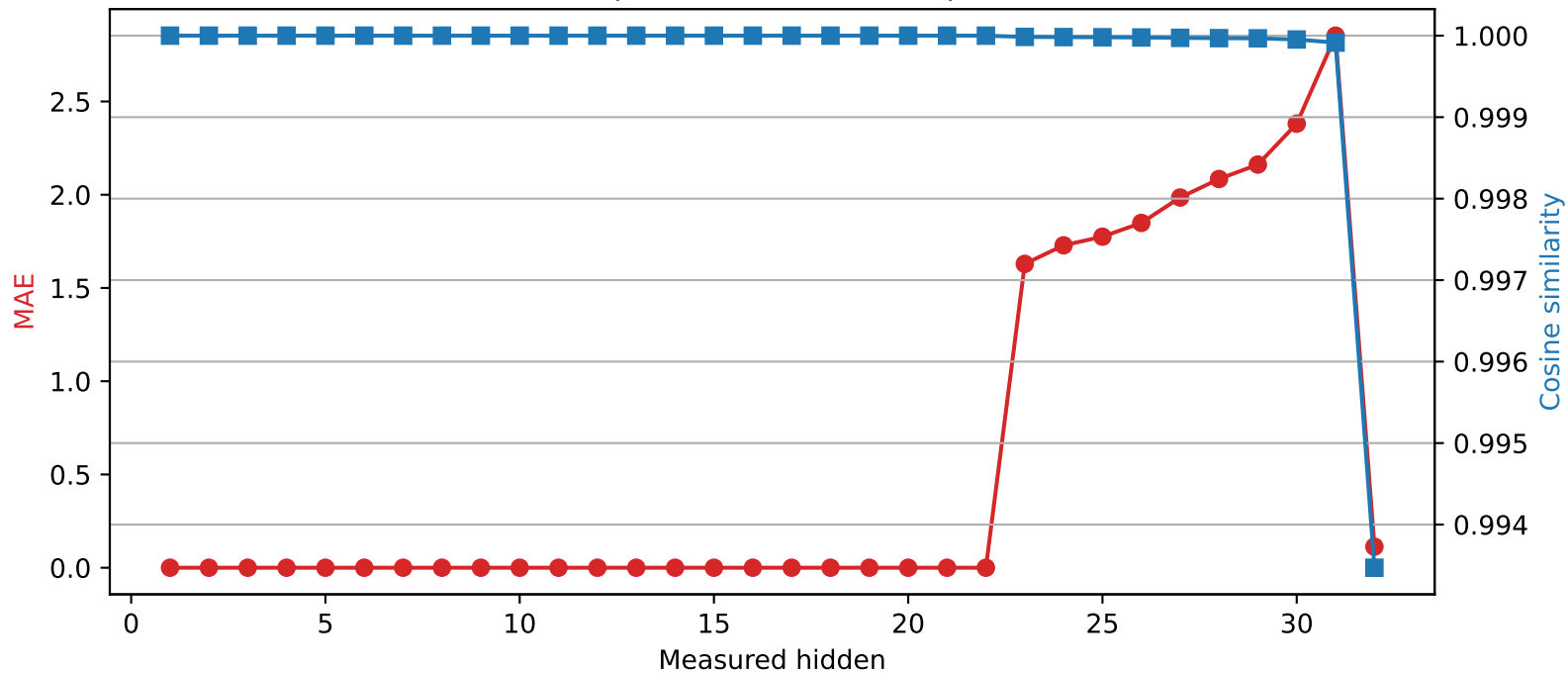
SmolLM2-360M | Quantized layer 22 | float64 → int2
