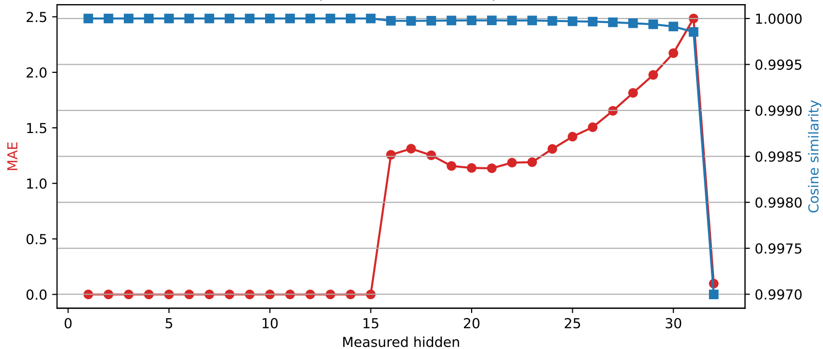
SmolLM2-360M | Quantized layer 15 | float64 → int2
