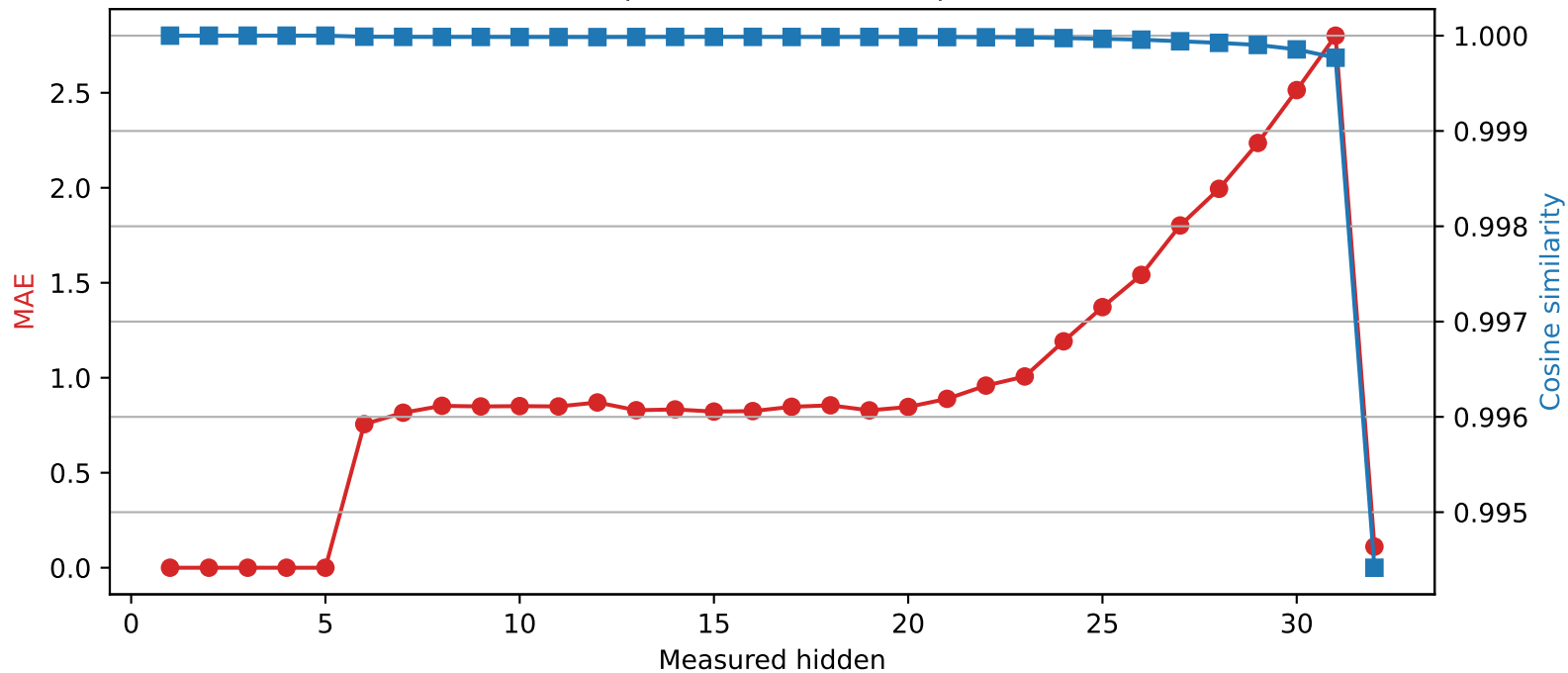
SmolLM2-360M | Quantized layer 5 | float64 → int2
