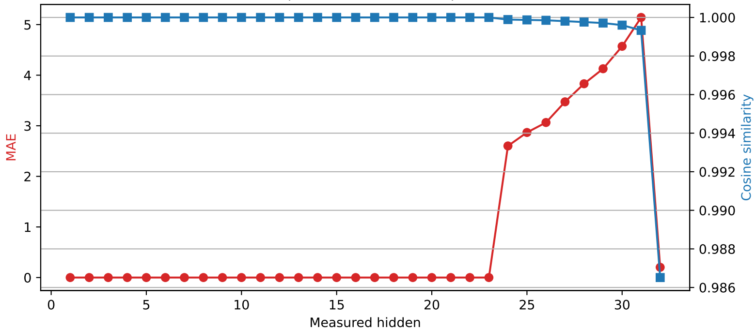
SmolLM2-360M | Quantized layer 23 | float64 → int2
