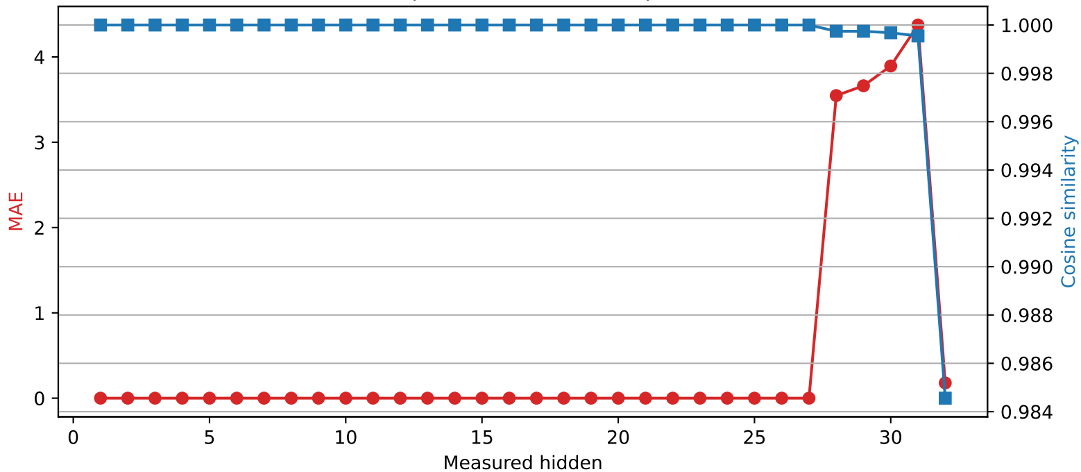
SmolLM2-360M | Quantized layer 27 | float64 → int2
