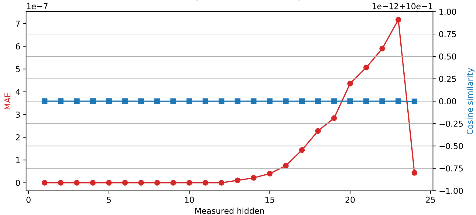
SmolLM2-1.7B-Instruct | Quantized layer 12 | float64 → int32
