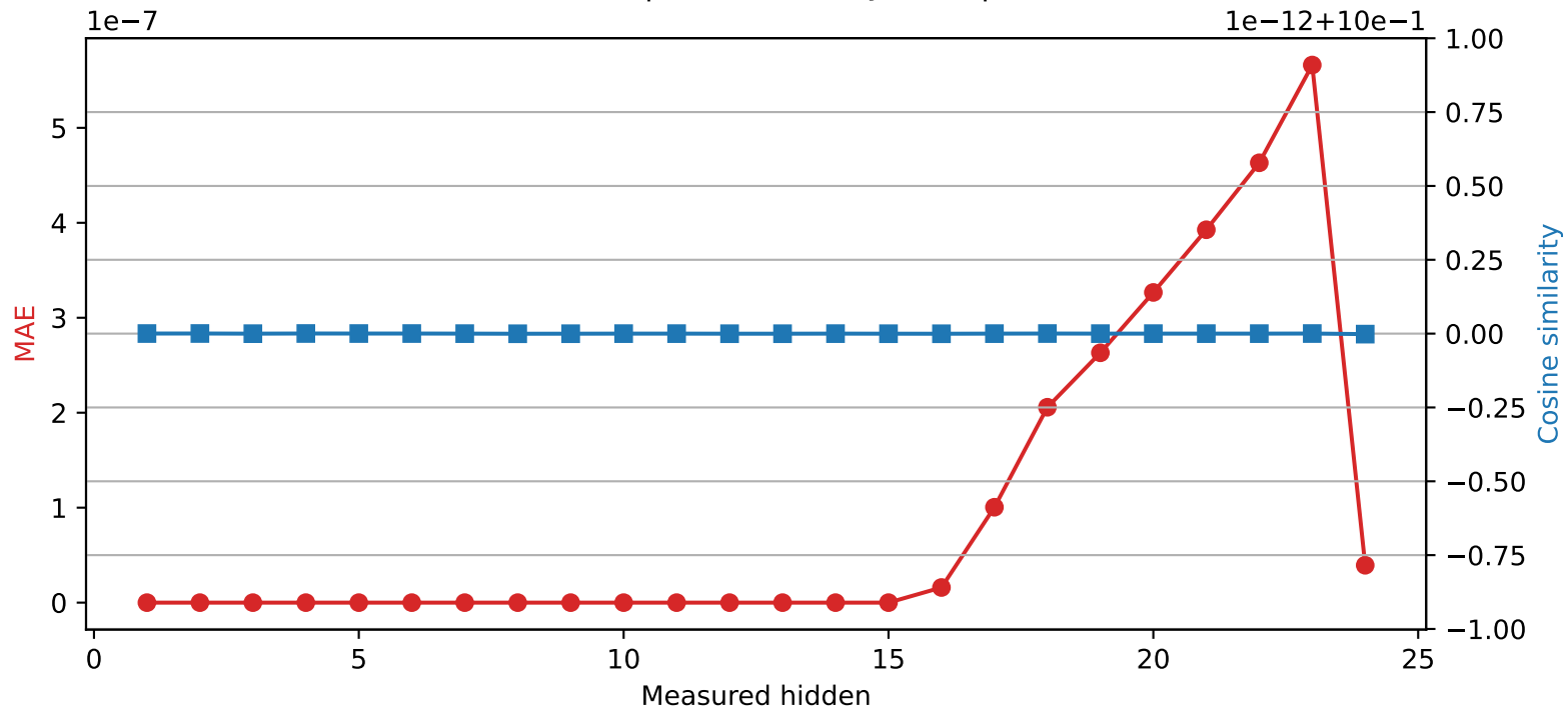
SmolLM2-1.7B-Instruct | Quantized layer 15 | float64 → int32
