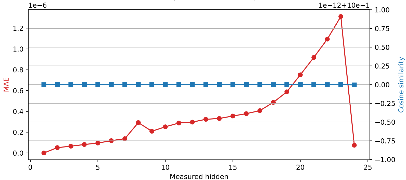
SmolLM2-1.7B-Instruct | Quantized layer 1 | float64 → int32
