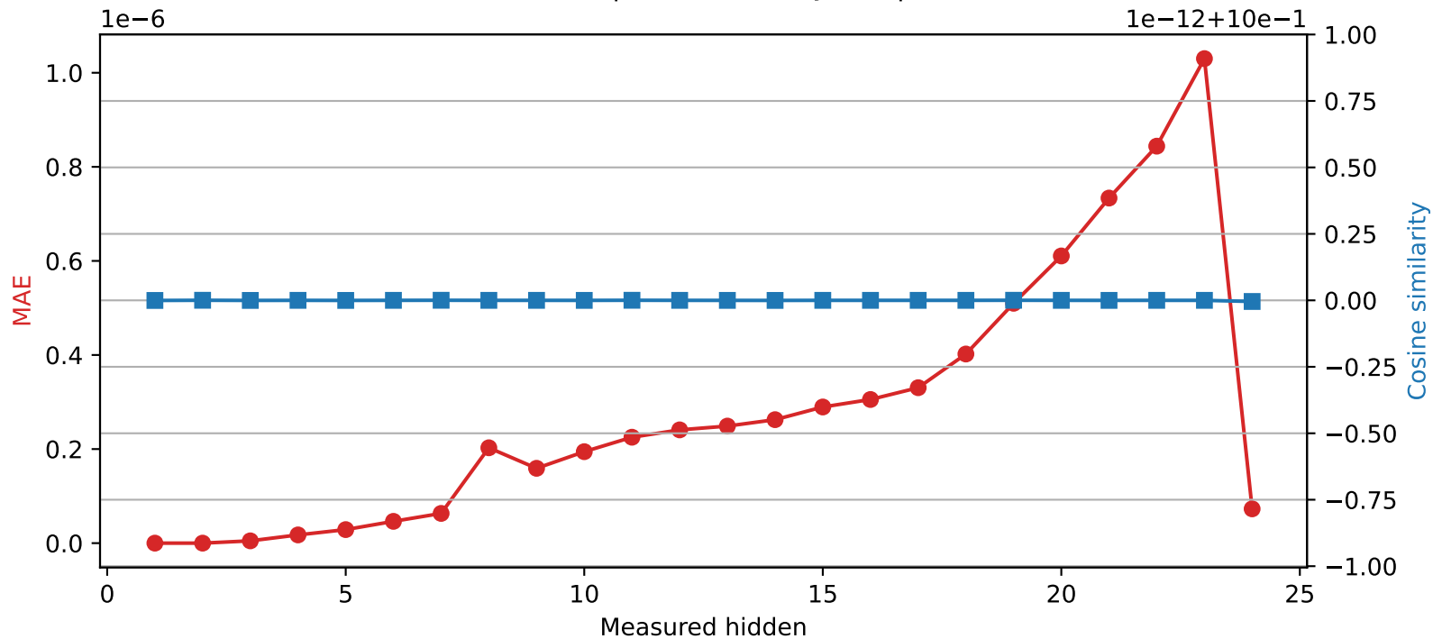
SmolLM2-1.7B-Instruct | Quantized layer 2 | float64 → int32
