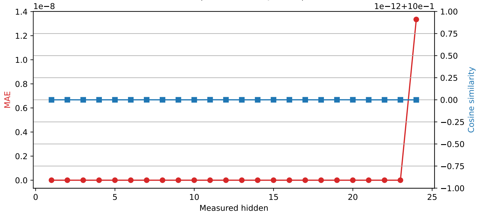
SmolLM2-1.7B-Instruct | Quantized layer 23 | float64 → int32
