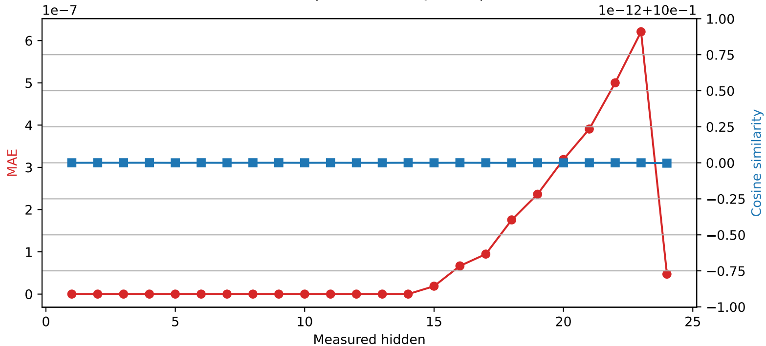
SmolLM2-1.7B-Instruct | Quantized layer 14 | float64 → int32
