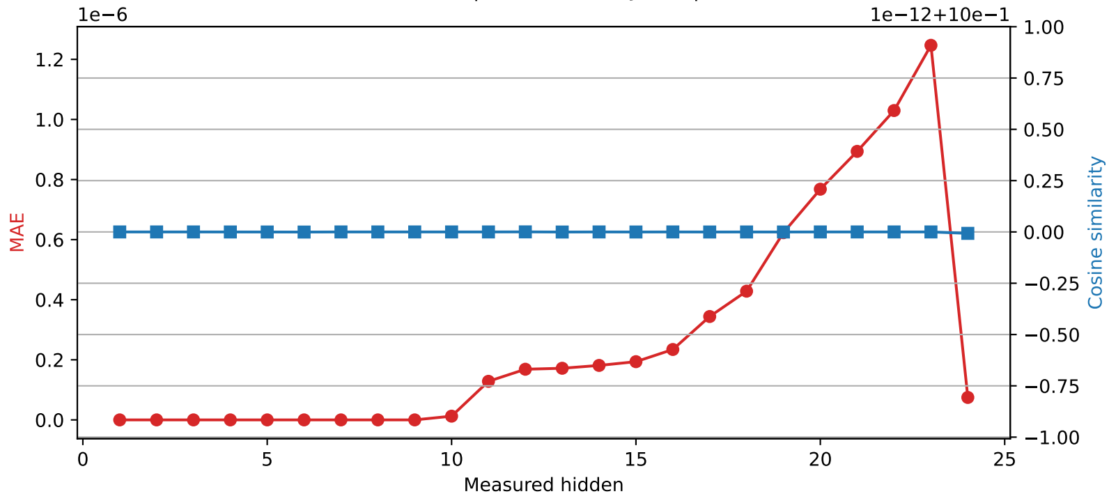
SmolLM2-1.7B-Instruct | Quantized layer 9 | float64 → int32
