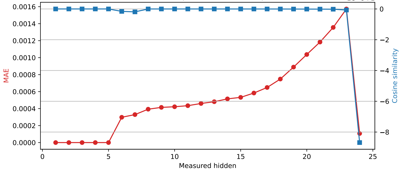
SmolLM2-1.7B-Instruct | Quantized layer 5 | float32 \rightarrow int16
