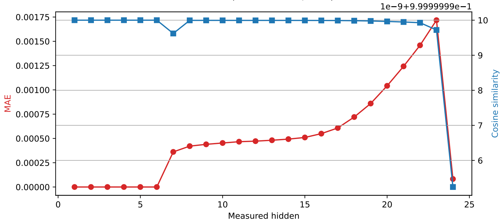
SmolLM2-1.7B-Instruct | Quantized layer 6 | float32 → int16
