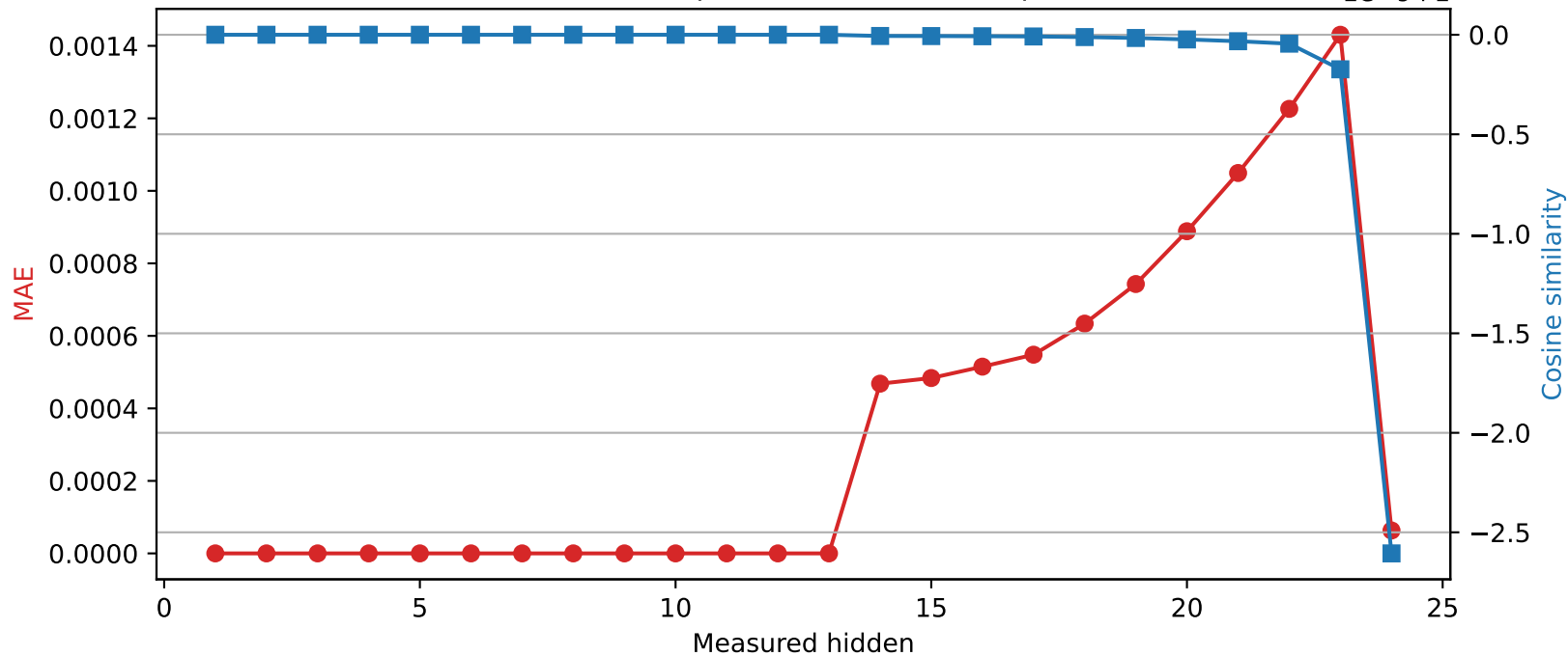
SmolLM2-1.7B-Instruct | Quantized layer 13 | float32 → int16
