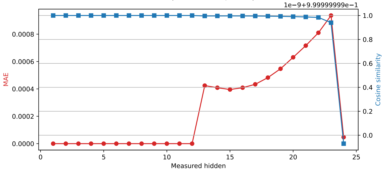
SmolLM2-1.7B-Instruct | Quantized layer 12 | float32 → int16
