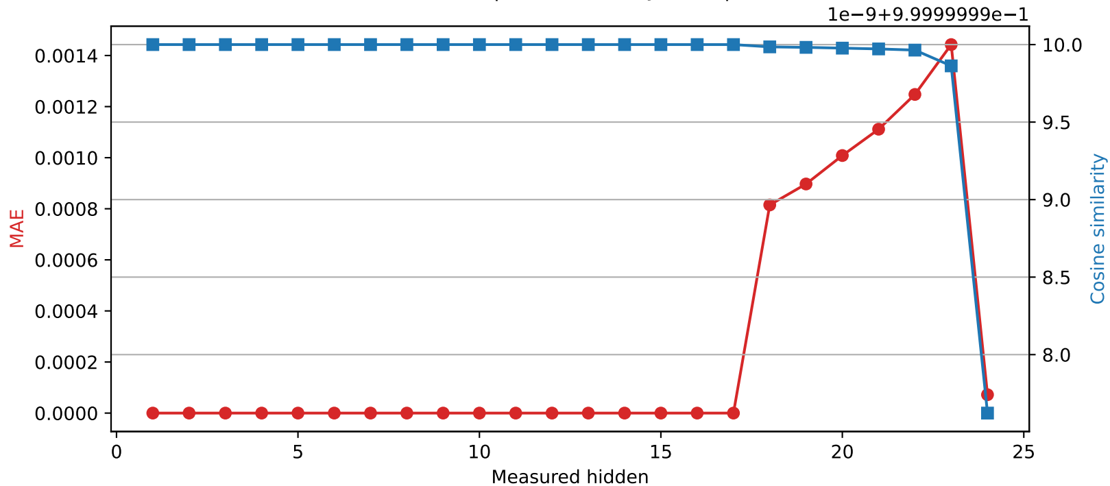
SmolLM2-1.7B-Instruct | Quantized layer 17 | float32 \rightarrow int16
