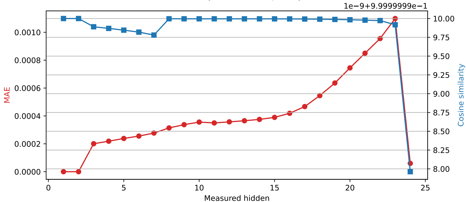
SmolLM2-1.7B-Instruct | Quantized layer 2 | float32 → int16
