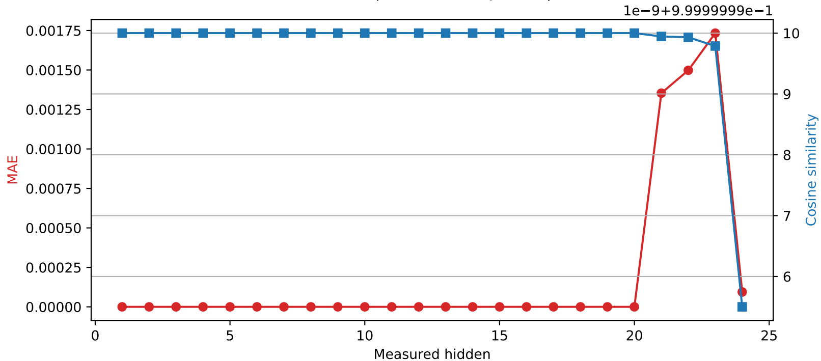
SmolLM2-1.7B-Instruct | Quantized layer 20 | float32 → int16
