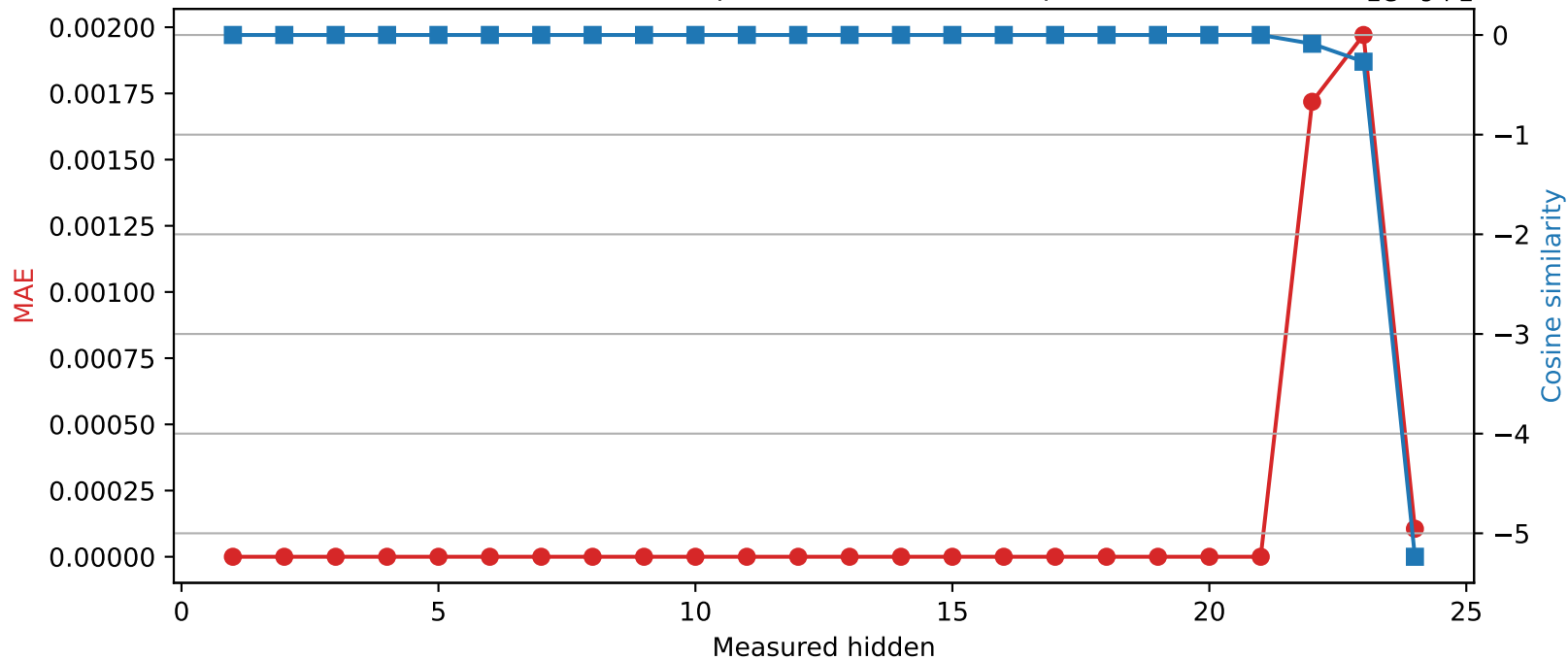
SmolLM2-1.7B-Instruct | Quantized layer 21 | float32 → int16
