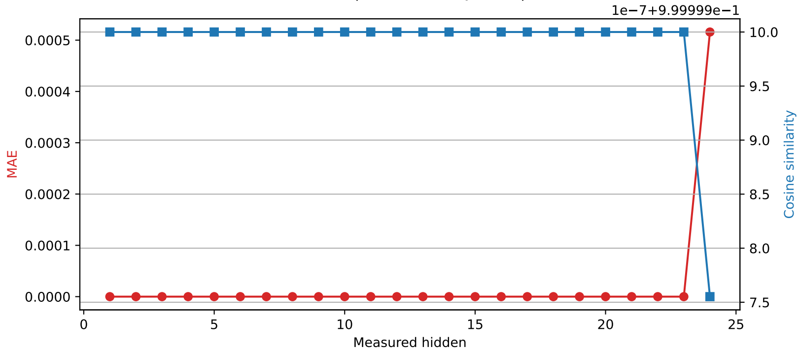
SmolLM2-1.7B-Instruct | Quantized layer 23 | float32 \rightarrow int16
