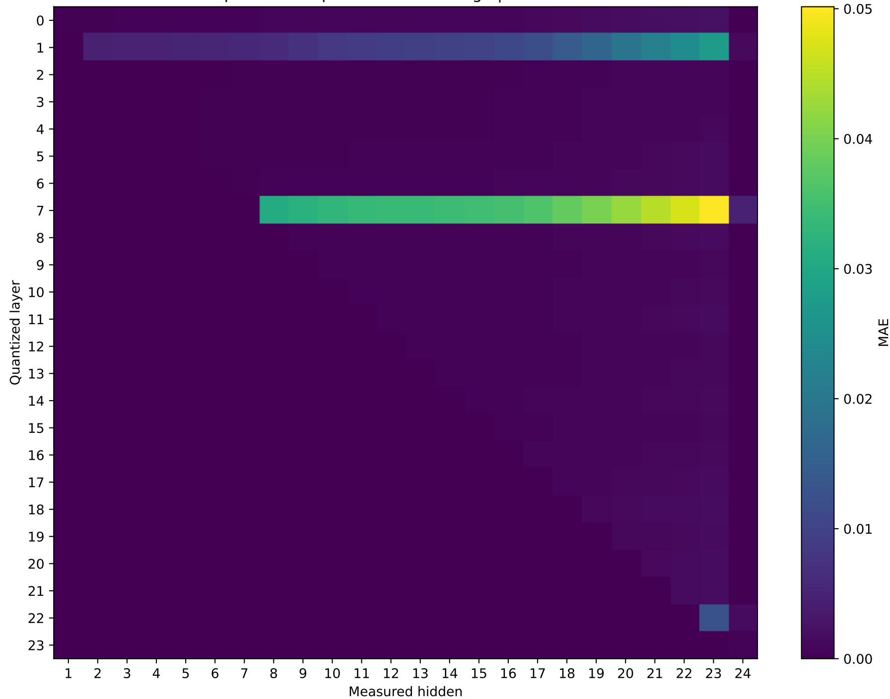
SmolLM2-1.7B-Instruct Prompt 4: MAE representation damage | float32 → int16
