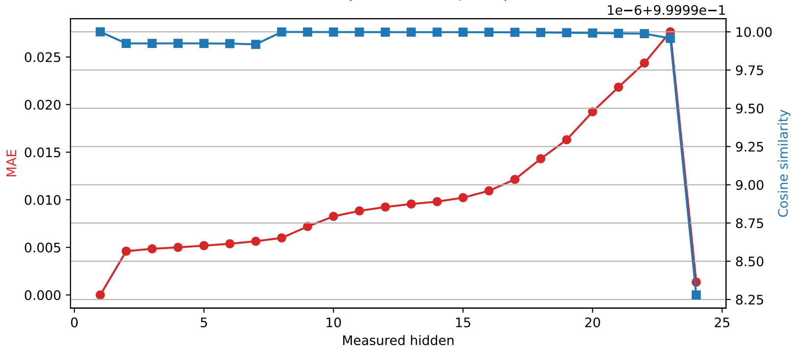
SmolLM2-1.7B-Instruct | Quantized layer 1 | float32 → int16
