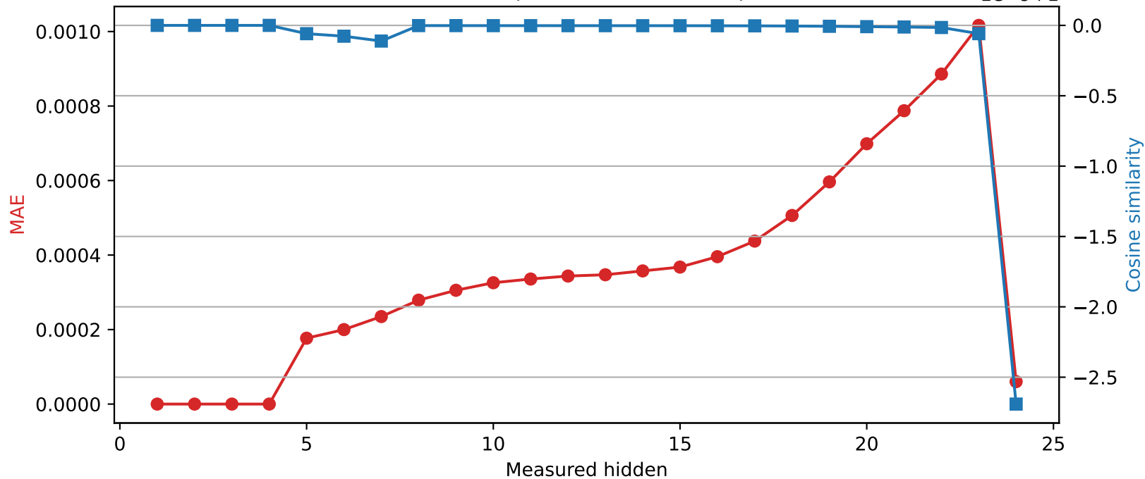
SmolLM2-1.7B-Instruct | Quantized layer 4 | float32 \rightarrow int16
