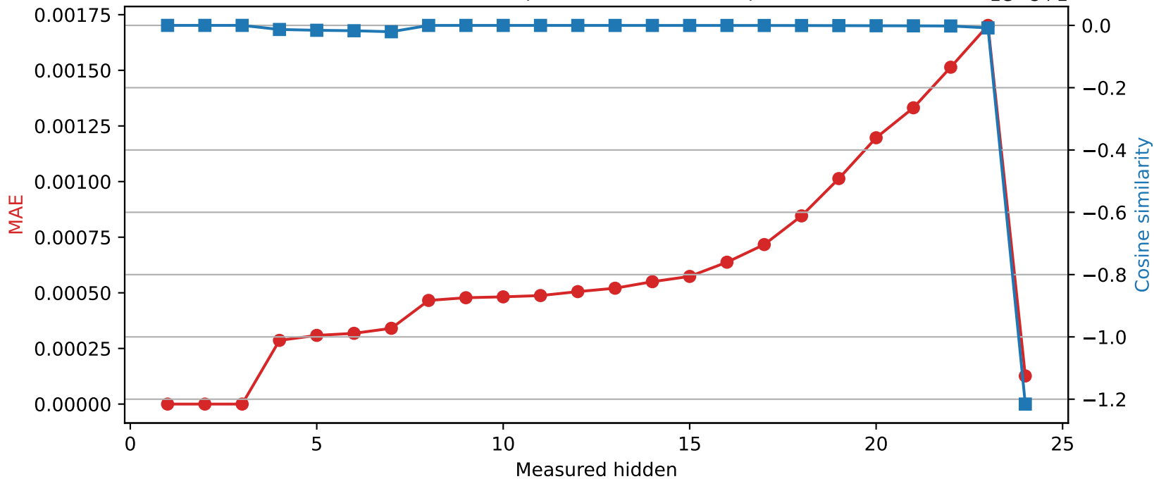
SmolLM2-1.7B-Instruct | Quantized layer 3 | float64 → int16
