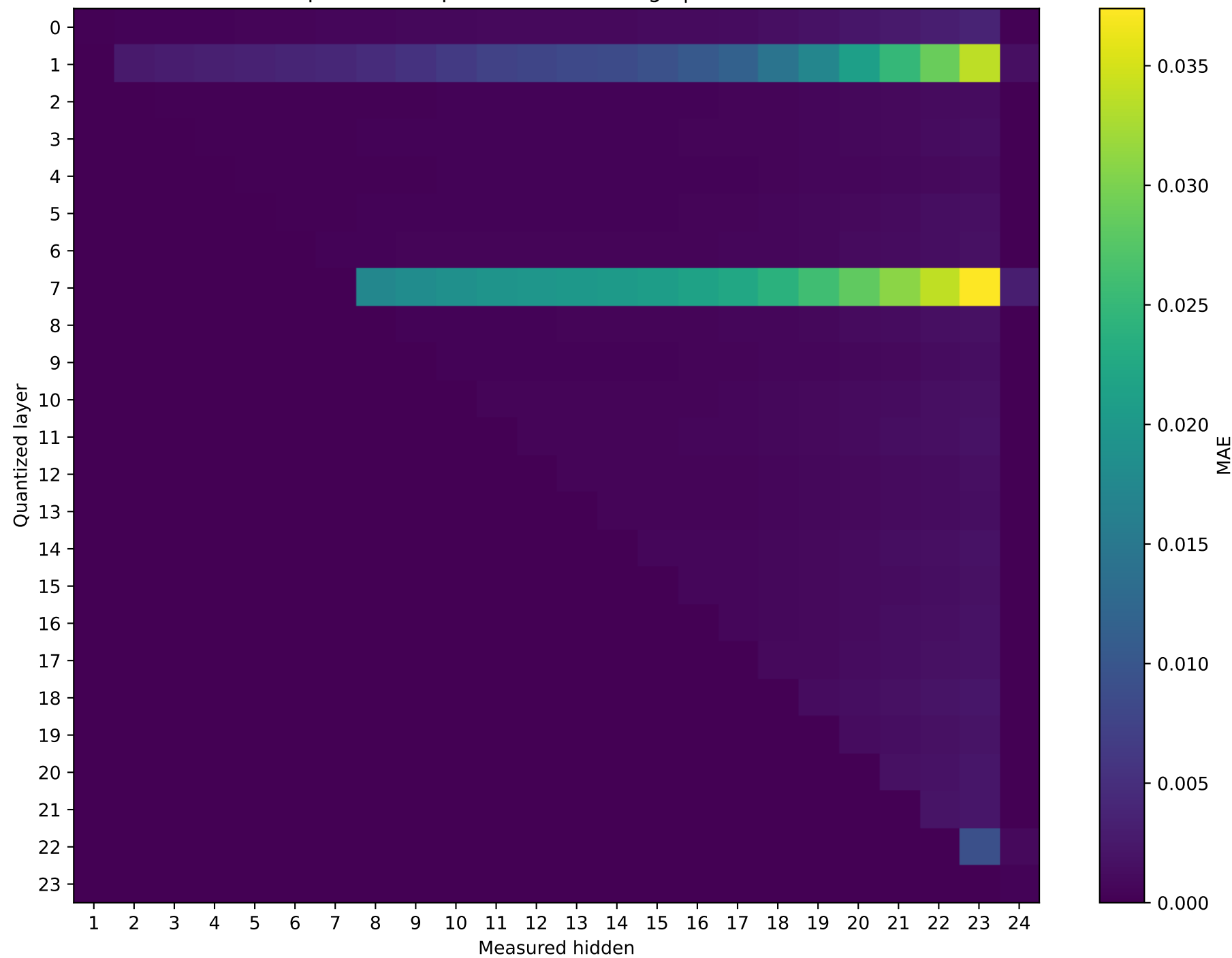
SmolLM2-1.7B-Instruct Prompt 1: MAE representation damage | float64 → int16
