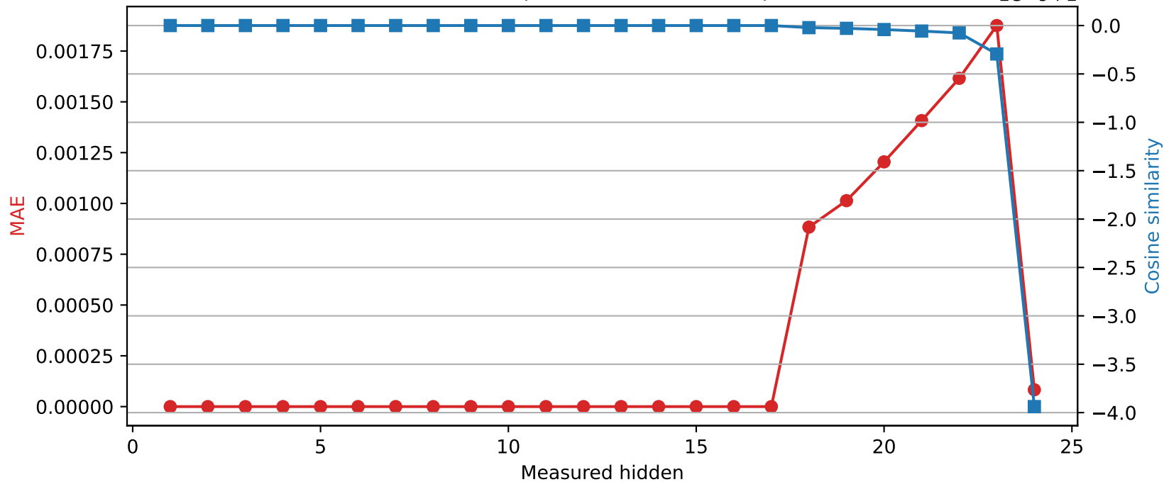
SmolLM2-1.7B-Instruct | Quantized layer 17 | float64 → int16
