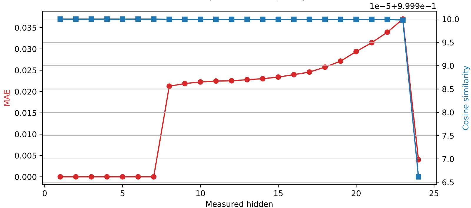
SmolLM2-1.7B-Instruct | Quantized layer 7 | float64 → int16
