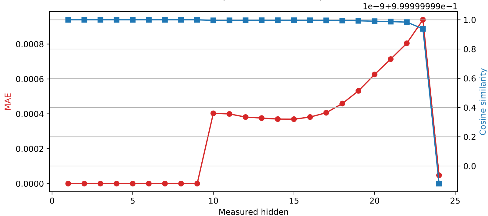
SmolLM2-1.7B-Instruct | Quantized layer 9 | float64 → int16
