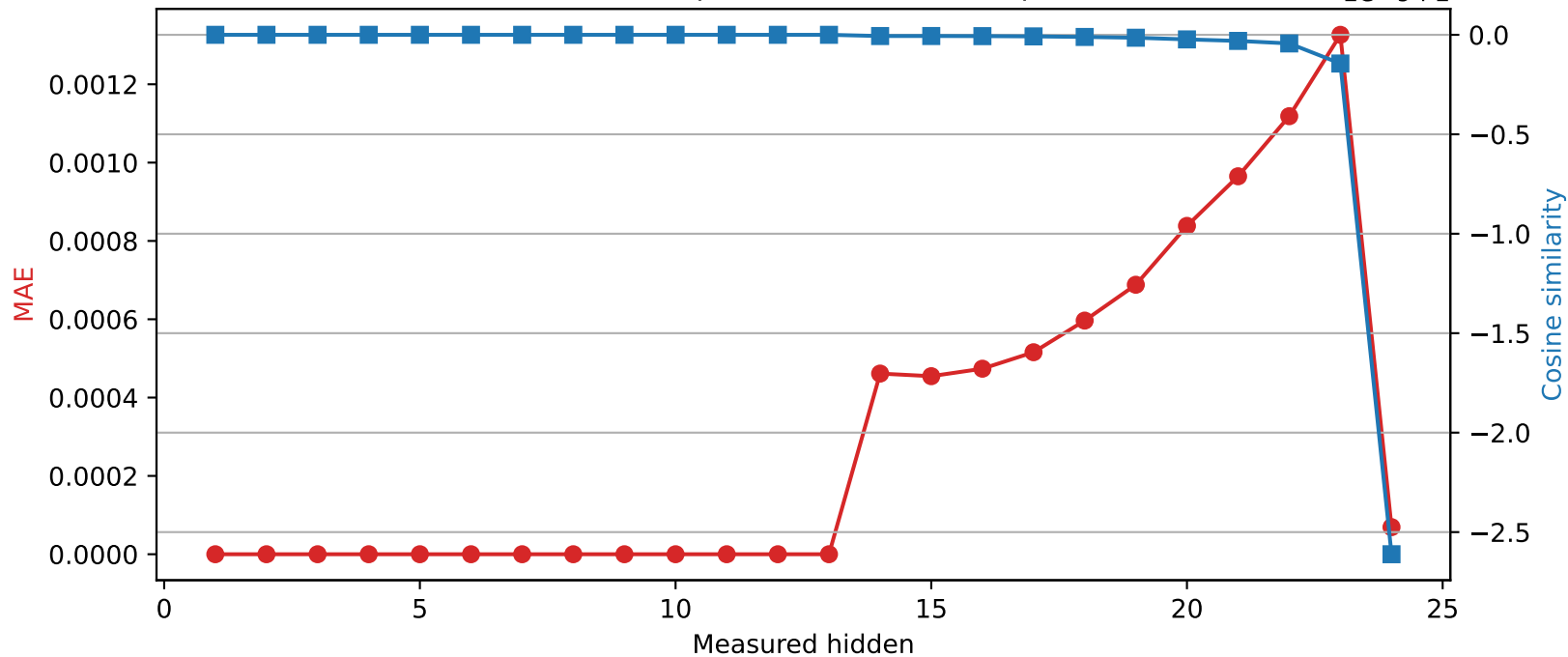
SmolLM2-1.7B-Instruct | Quantized layer 13 | float64 → int16
