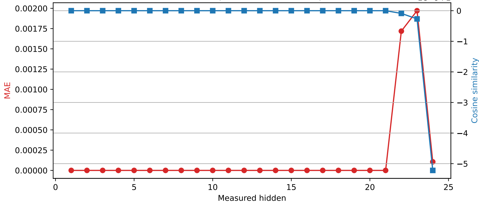
SmolLM2-1.7B-Instruct | Quantized layer 21 | float64 → int16
