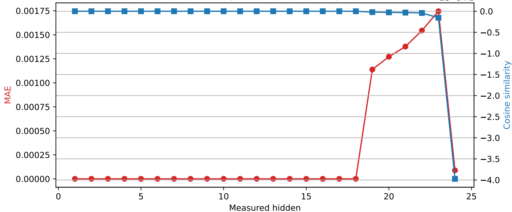
SmolLM2-1.7B-Instruct | Quantized layer 18 | float64 → int16
