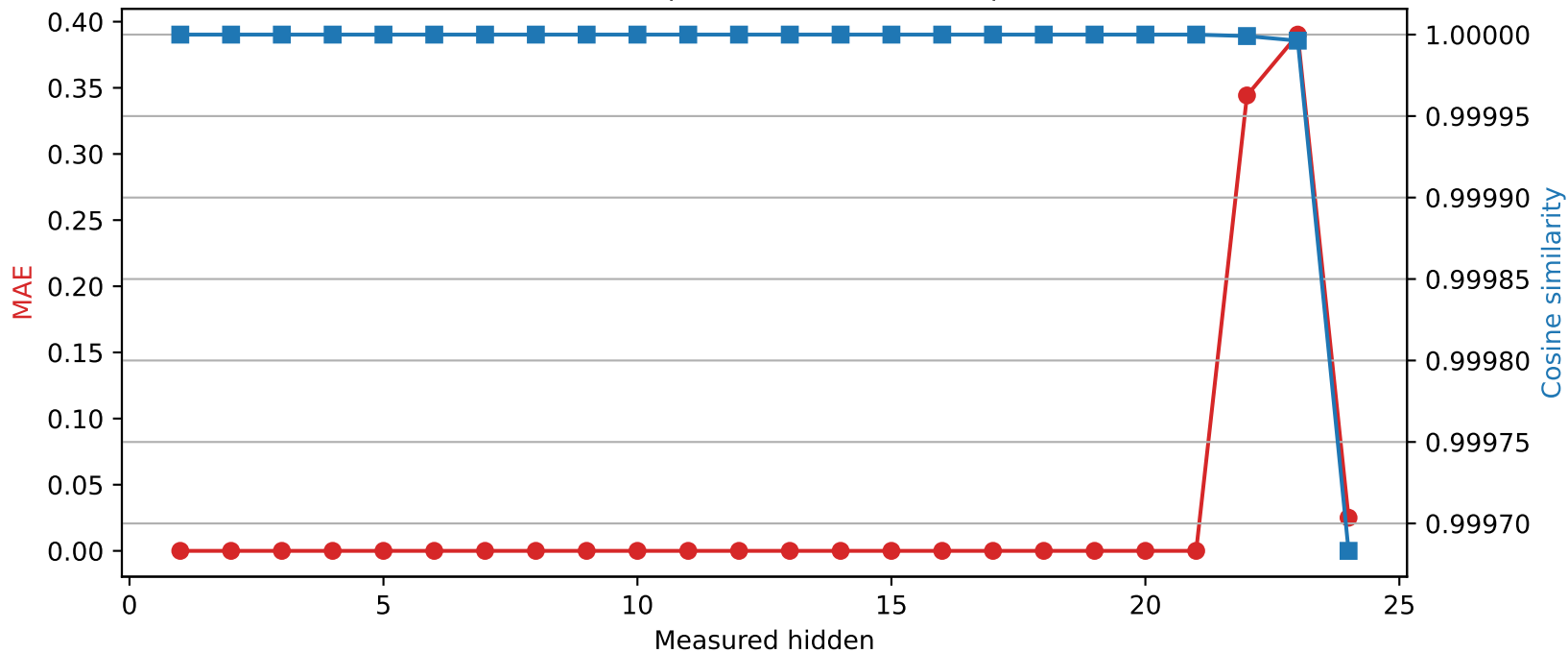
SmolLM2-1.7B-Instruct | Quantized layer 21 | float16 \rightarrow int8
