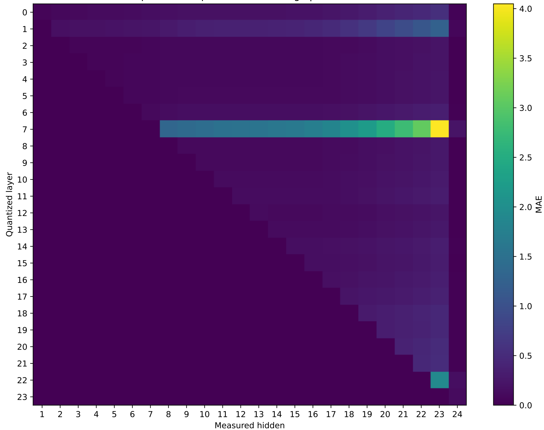
SmolLM2-1.7B-Instruct Prompt 2: MAE representation damage | float16 \rightarrow int8
