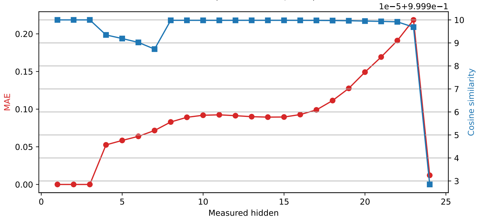
SmolLM2-1.7B-Instruct | Quantized layer 3 | float16 → int8
