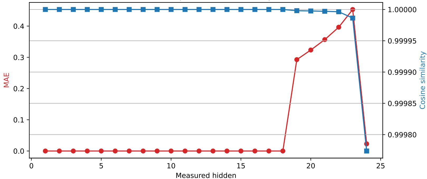
SmolLM2-1.7B-Instruct | Quantized layer 18 | float16 \rightarrow int8
