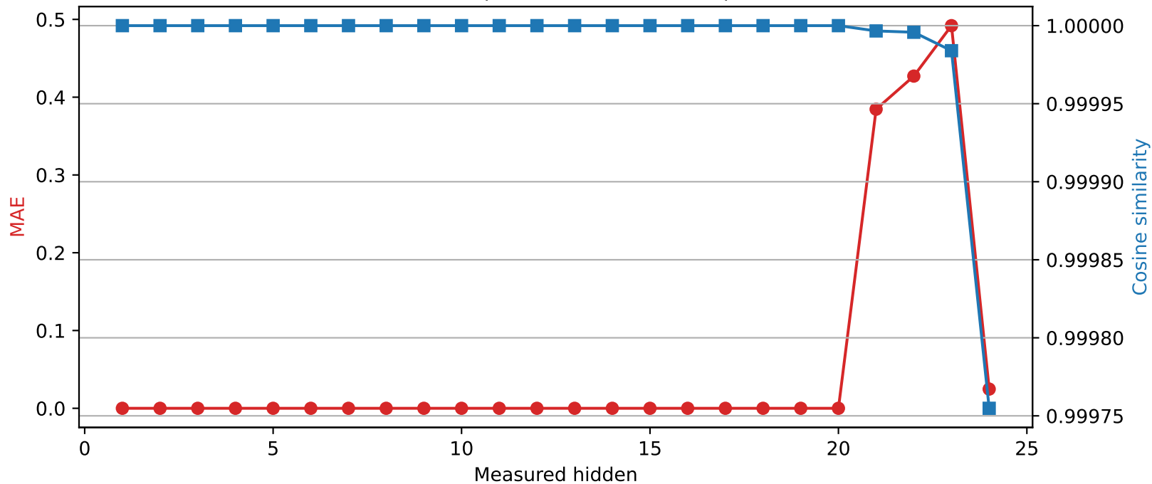
SmolLM2-1.7B-Instruct | Quantized layer 20 | float16 \rightarrow int8
