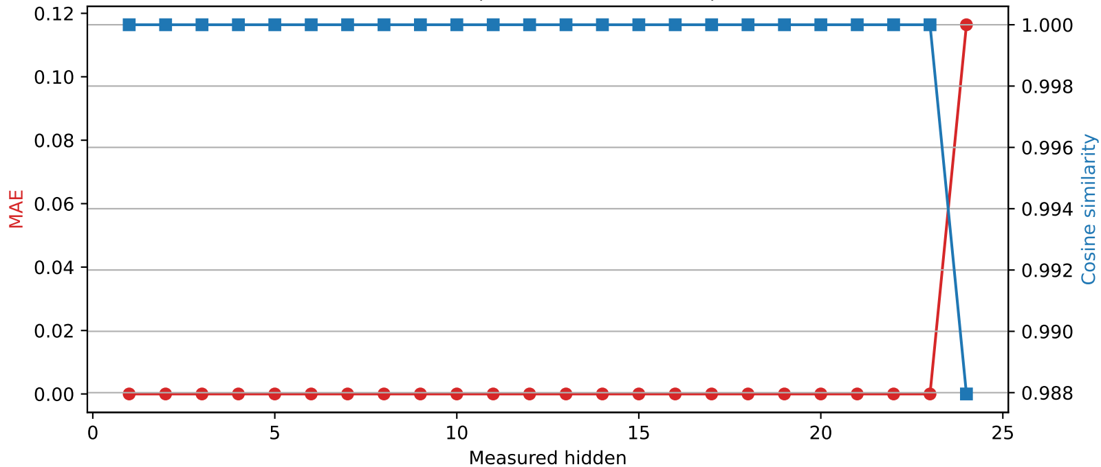
SmolLM2-1.7B-Instruct | Quantized layer 23 | float16 → int8
