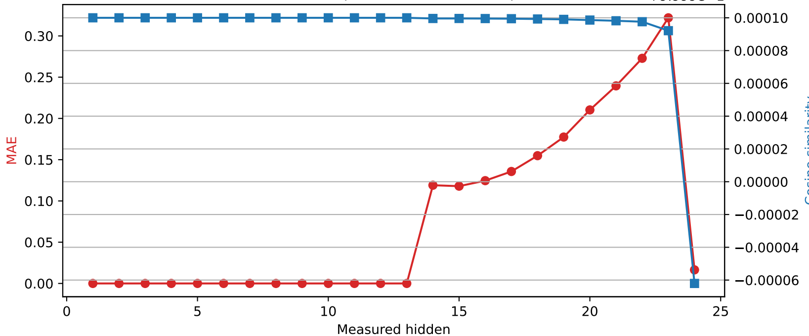
SmolLM2-1.7B-Instruct | Quantized layer 13 | float16 \rightarrow int8
